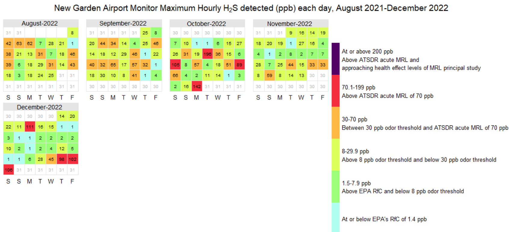
Figure C11 (Continued). New Garden Airport Monitor Maximum Hourly H 2 S concentrations (ppb) by date. Days that are blank/white = not enough data to be considered (less than 80% of valid hours on that date). Figure was prepared using the openair package in R.
