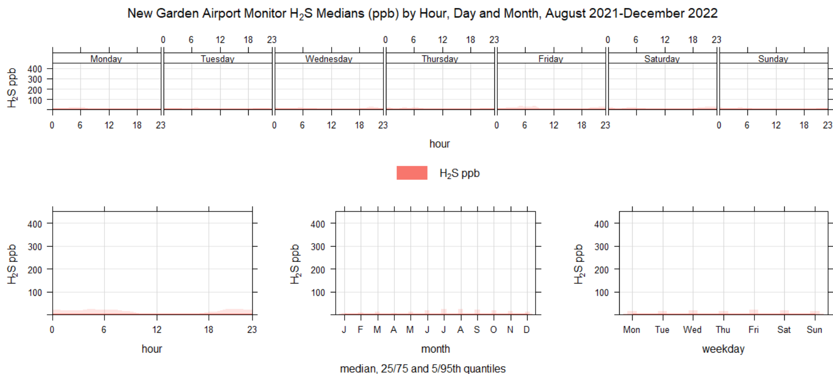
Figure C8. New Garden Airport Monitor H 2 S medians (ppb) by hour of day, day of week, and month of year. The same y-axis scale is shown for this monitor as for the Landenberg (Figure C6) and West Grove Monitor (Figure C7). The data show that 95 th percentiles (represented by the light pink shading) of the Airport data were much lower than the 95 th percentiles of the two near-source monitors. Medians plotted below encompass days with 80% or more valid data (20 hours or more). Figure was prepared using the openair package in R.
