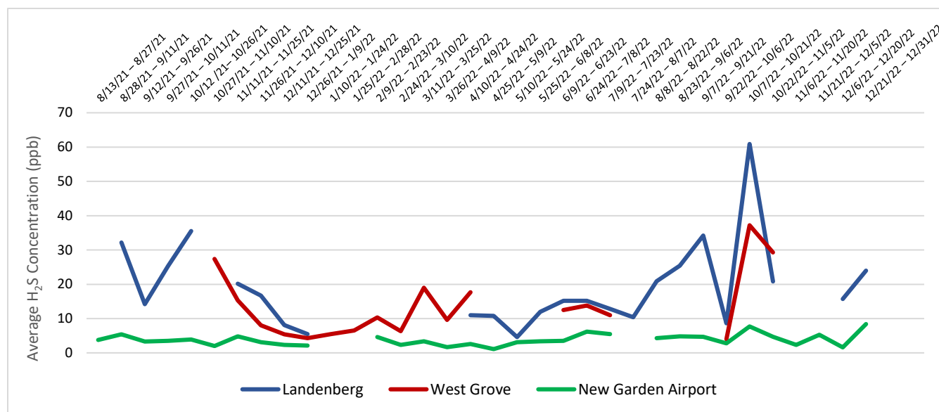
Figure 4. 15-Day H 2 S average concentrations (ppb) at each monitor, August 2021–December 2022
