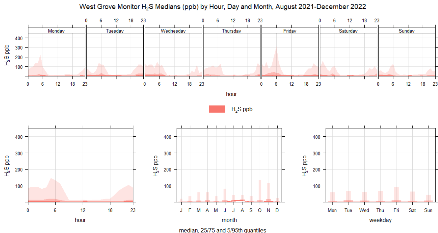
Figure C7. West Grove Monitor H 2 S medians (ppb) by hour of day, day of week, and month of year. The data show that compared to averages (Figures C5), medians (represented by the solid lines) were low. However, 95 th percentiles of the data were much higher (represented by the lightest pink shading) and these peaks occurred in the very early morning or nighttime hours, on Fridays, and in October and November. Medians plotted below encompass days with 80% or more valid data (20 hours or more). Figure was prepared using the openair package in R.
