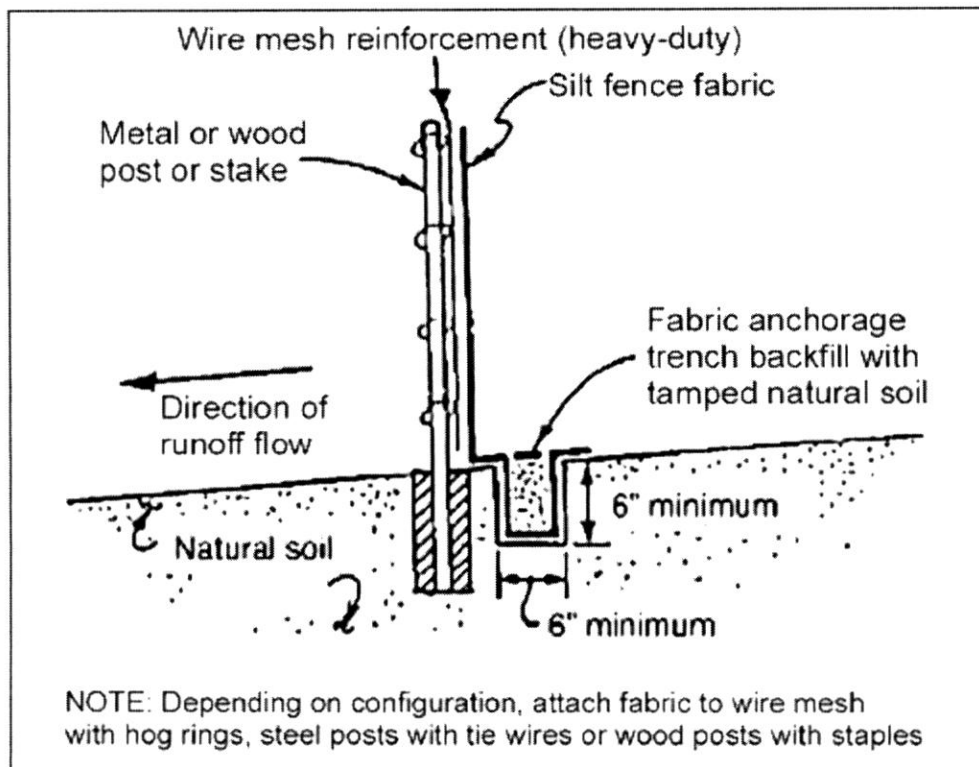
Figure 1: Typical Installation for Silt Fence
